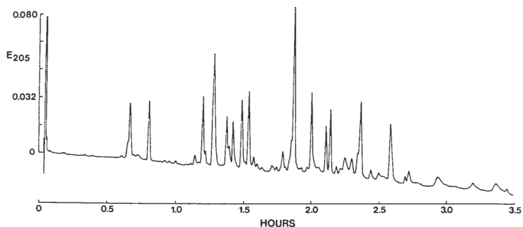
Figure 6 Separation of Thermus aquaticus 30S ribosomal proteins by reversed phase chromatography. Conditions as in Figure 4.
